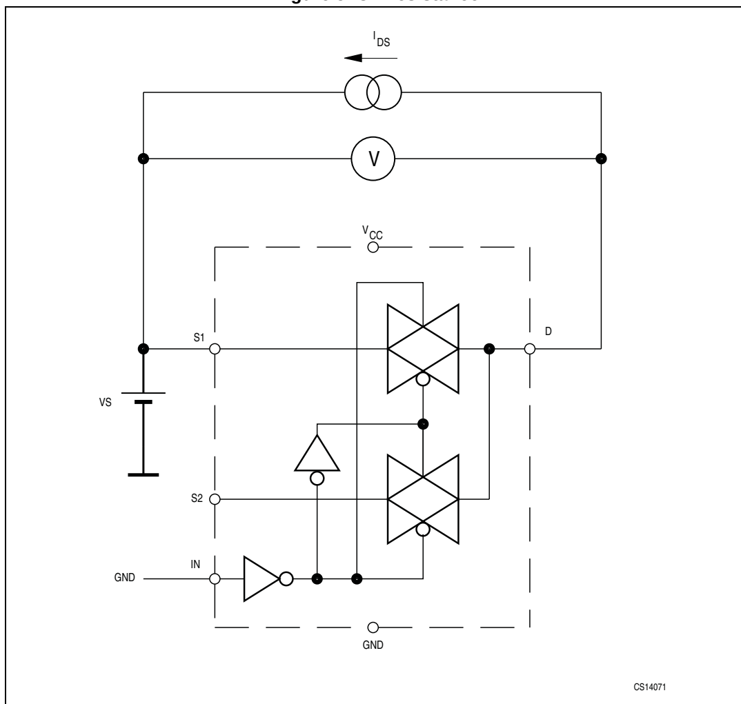
Figure 5. ON resistance
