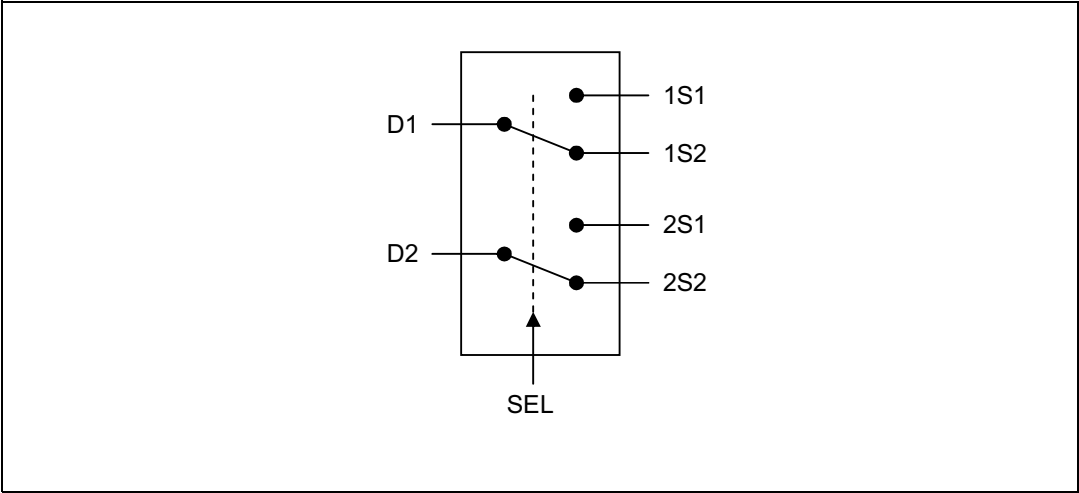
Figure 2. Logic block diagram
