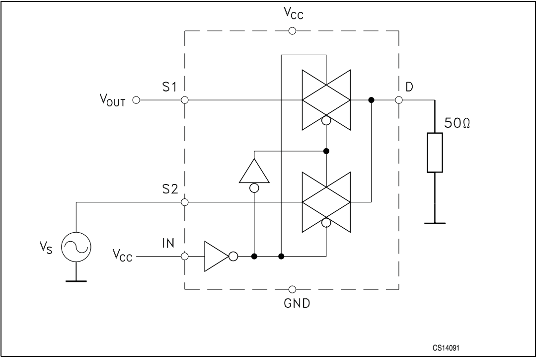
Figure 9. Channel-to-channel crosstalk
