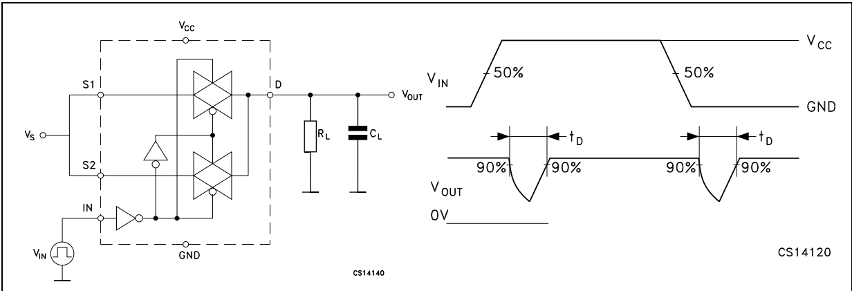
Figure 12. Switching time and charge injection ( V_{GEN} = 0\text{ V} , R_{GEN} = 0\text{ }\Omega , R_L = 1\text{ M}\Omega , C_L = 100\text{ pF} )
